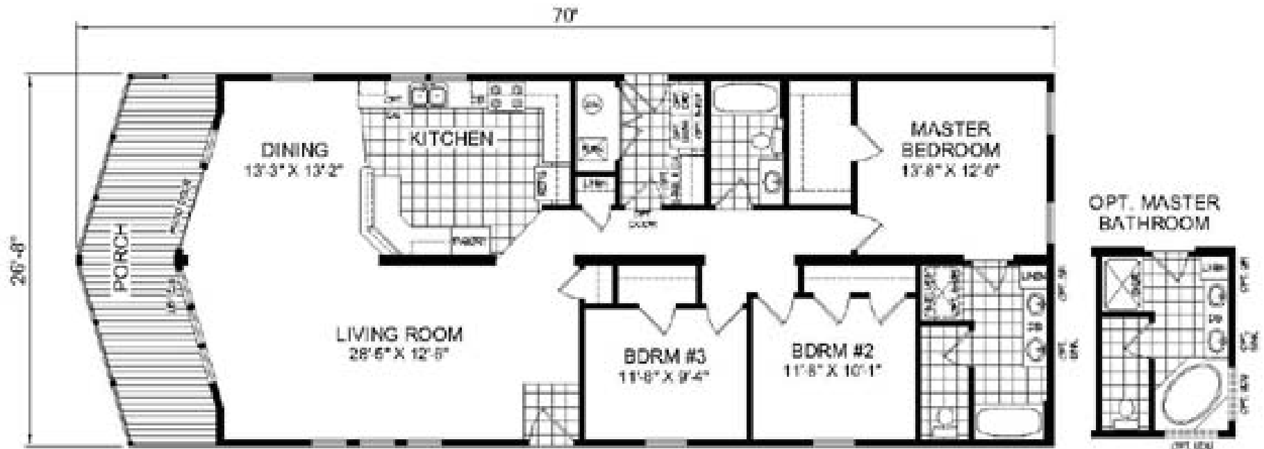
MODEL 655 3 BEDROOMS, 2 BATHS 1633.0 SQ. FT
